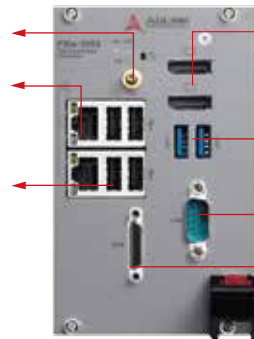
PXle-3985 Front Panel
